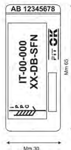
VERTICAL SIDE
